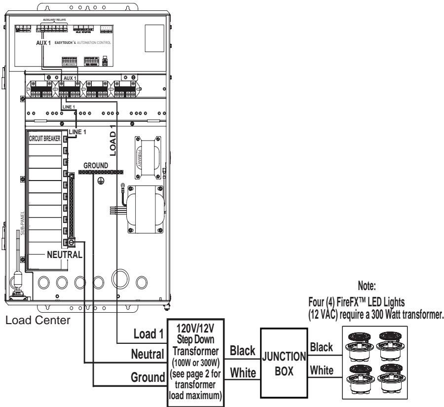
FireFX LED Light to EasyTouch or IntelliTouch Control System Load Center Wiring Connection Diagram
