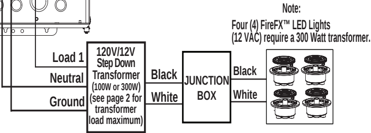
FireFX LED Light to EasyTouch or IntelliTouch Control System Load Center Wiring Connection Diagram
