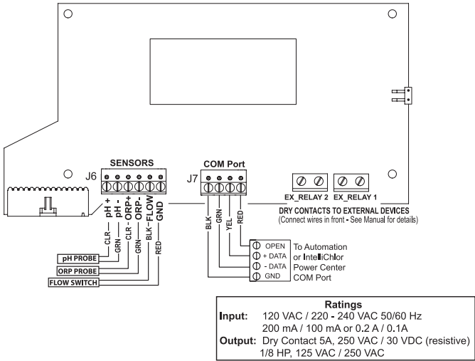
Figure 2: IntelliChem® Controller J6/J7 Circuit Board Wiring
