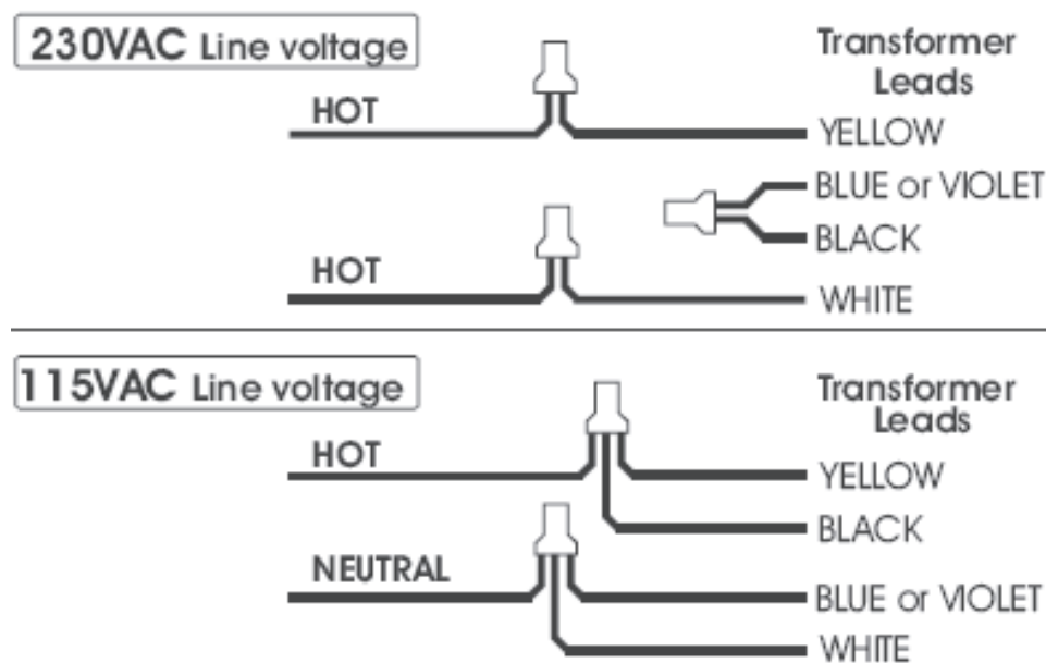
IntelliChlor Power Center 230 and 115 VAC Transformer Wiring
