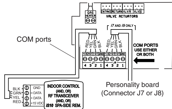
IntelliTouch Personality Circuit Board
