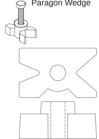
PW-Paragon Wedge Paragon Wedge
