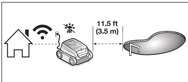
Figure 16. Charging Distance to Pool Edge
