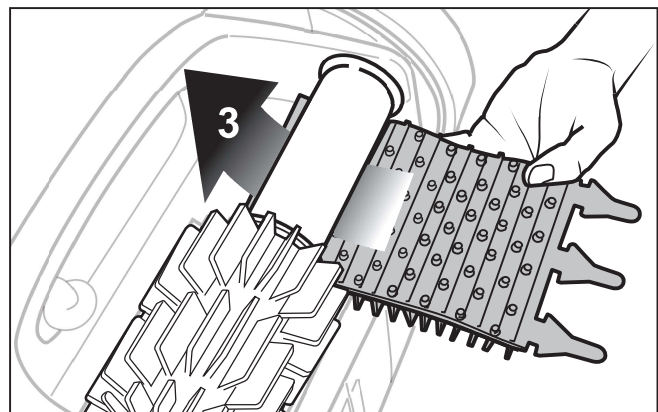
Figure 22. Install the New Brush
