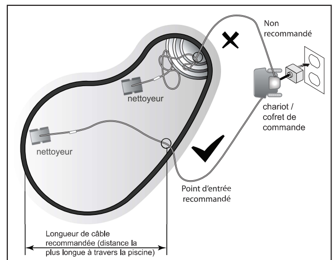
Figure 17. Configuration optimale
