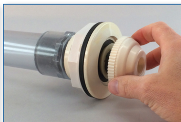
Install the face plate
