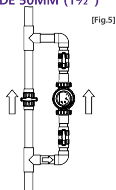
Installation verticale
