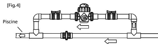
Installation horizontale
