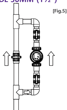
Installation verticale
