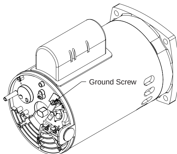
Figure 1. Field Wiring Compartment
