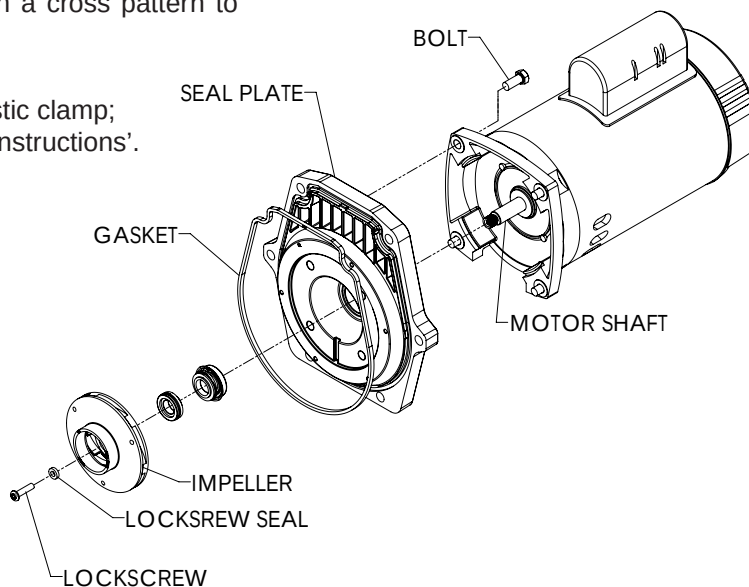
Motor Assembly
