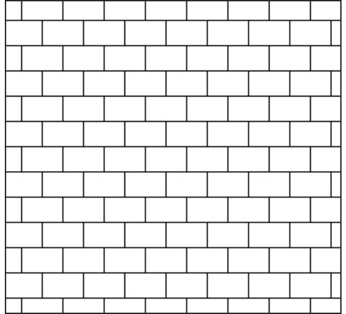
RUNNER BOND (7)
