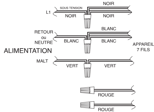
Figure 32. Raccordements à 120 VCA
