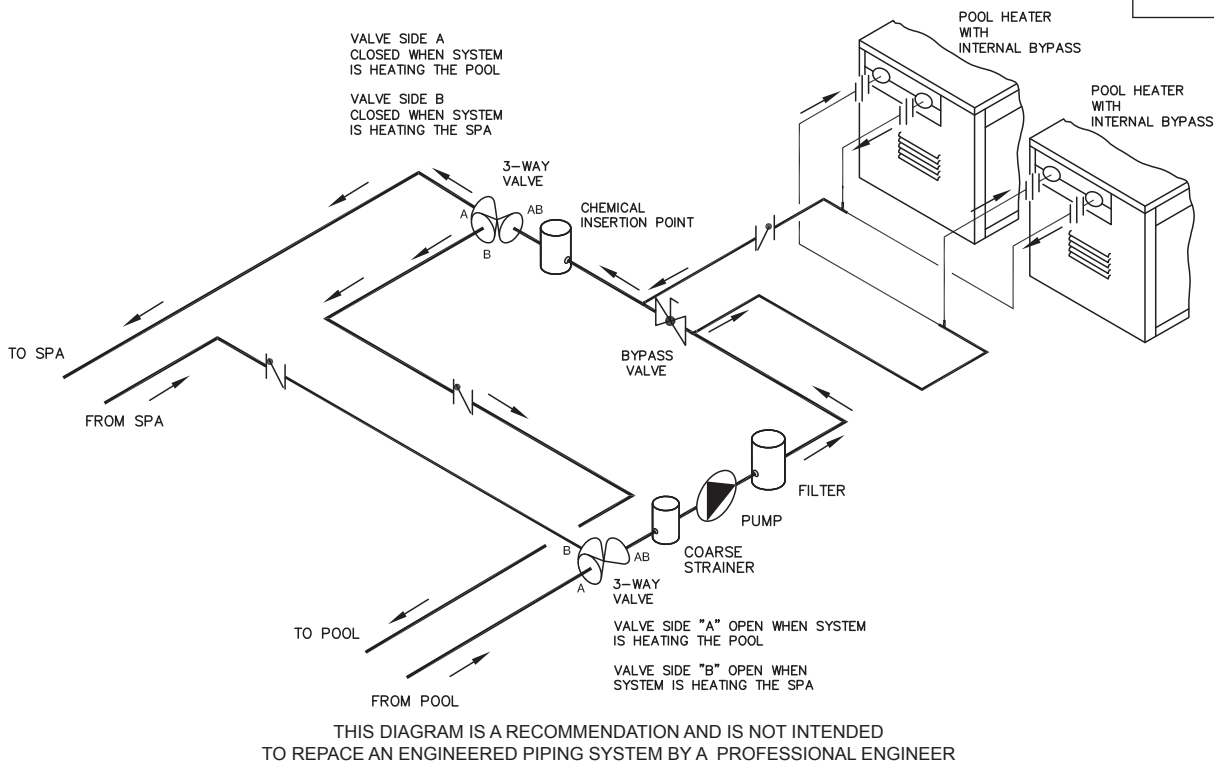
Figure 30. Multiple Pool Heater Installation
