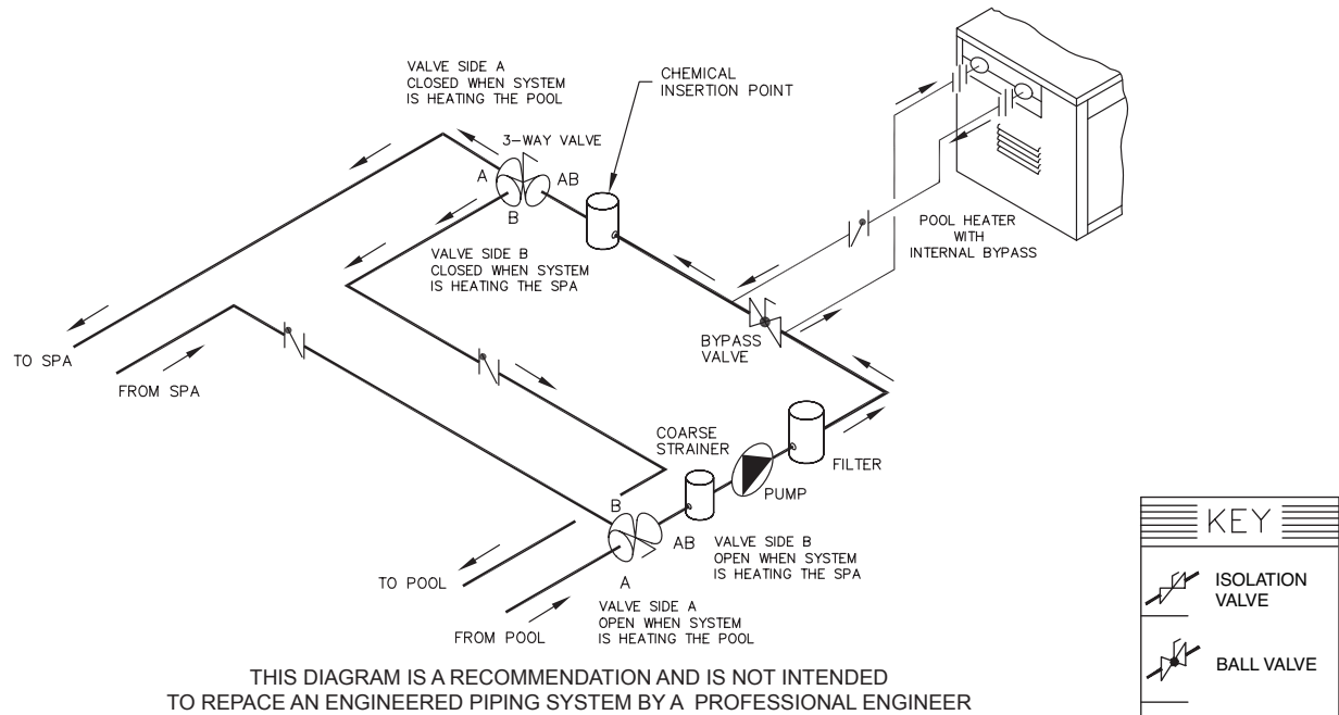
Figure 29. Single Pool Heater Installation
