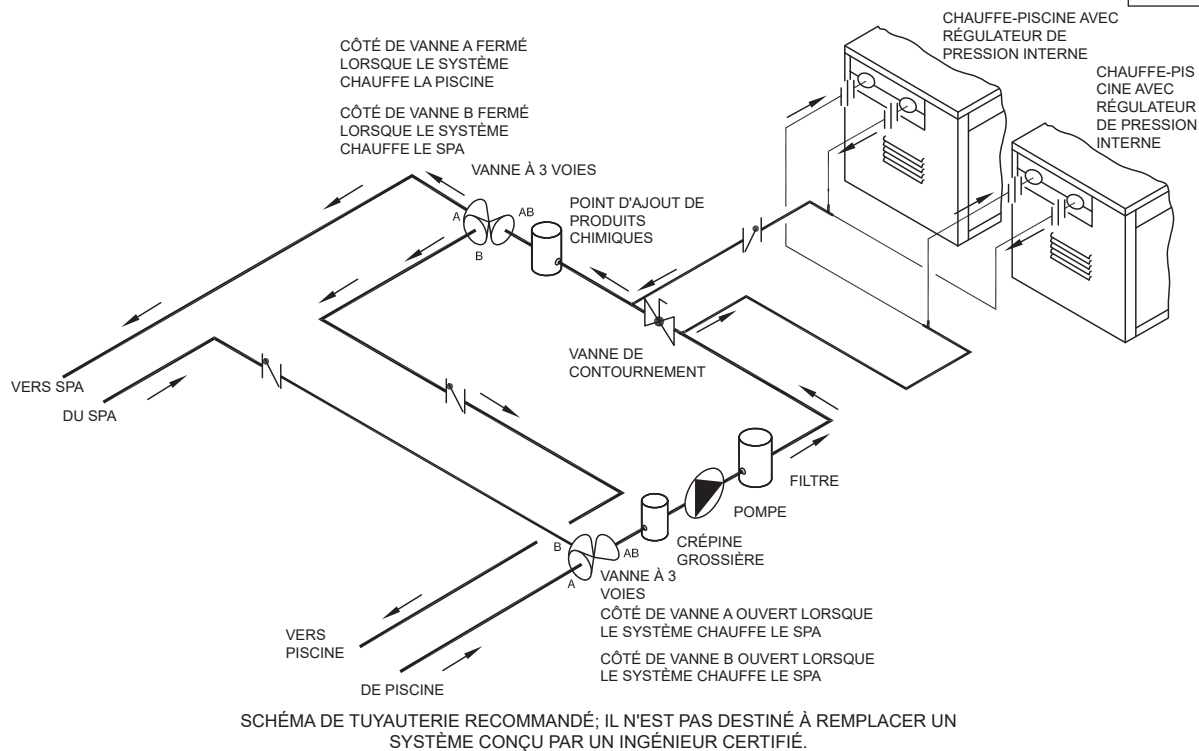
Figure 30. Installation, multi-appareils de chauffage
