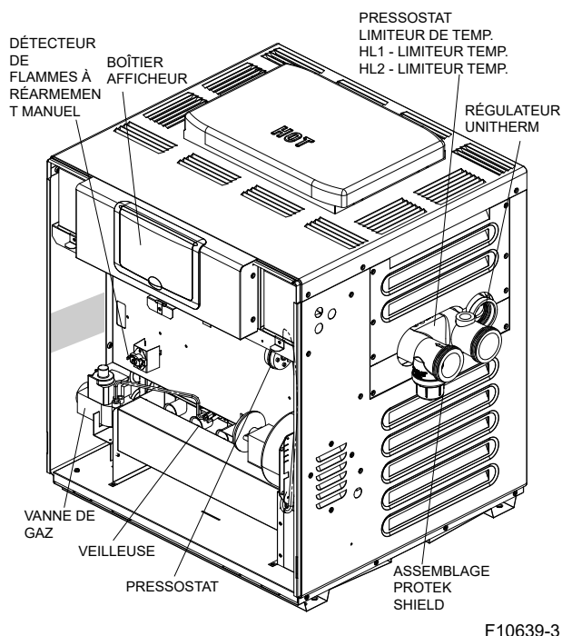
Figure 34. Emplacement des commandes (1)
