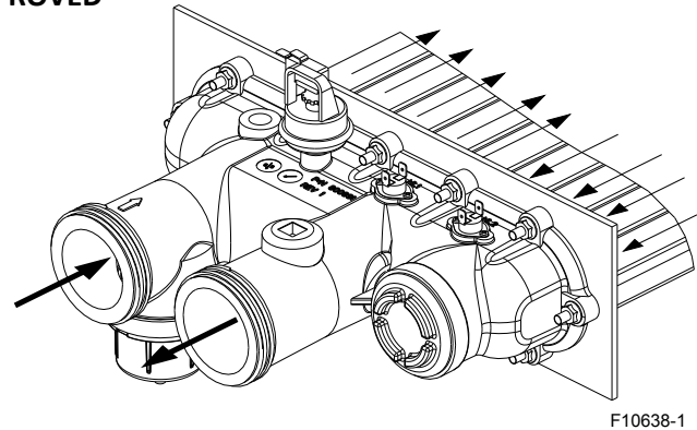
Figure 15. Polymer Headers Water Flow
