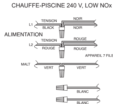
Figure 33. Raccordements à 240 VCA
