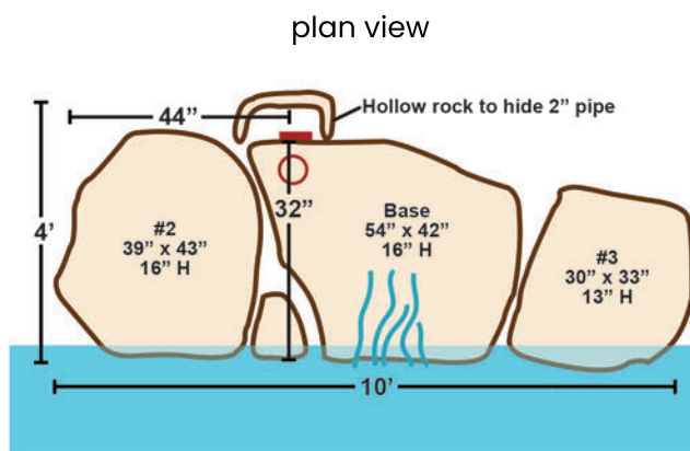
6" plumbing sleeve for 2" pipe should be filled with spray foam or mortar after pipe is set
