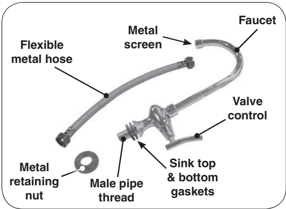
Fig. 1-1 Faucet detail
