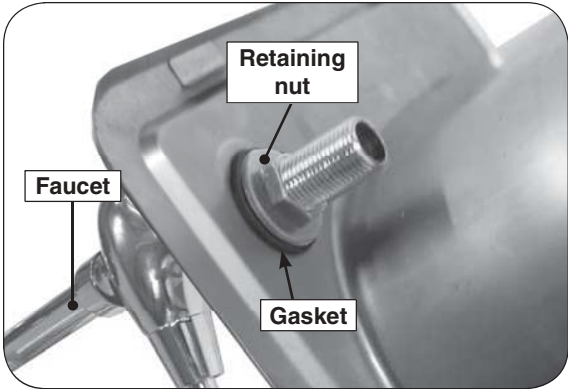
Fig. 1-2 Tighten retaining nut
