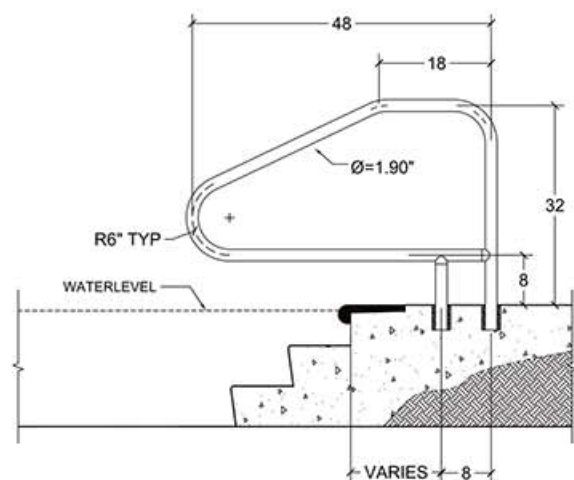
RETURN-TO-DECK HANDRAIL CBRTD-448 CROSS BRACED
