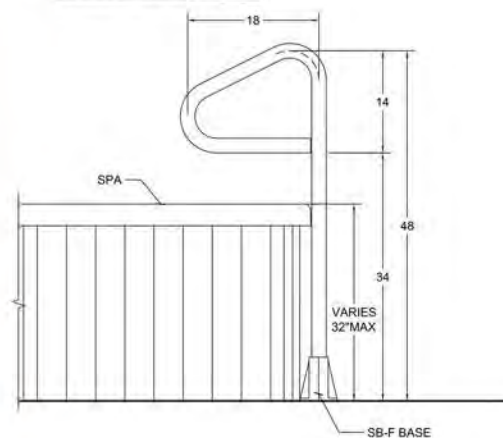
SF-48 SPA RAILS
