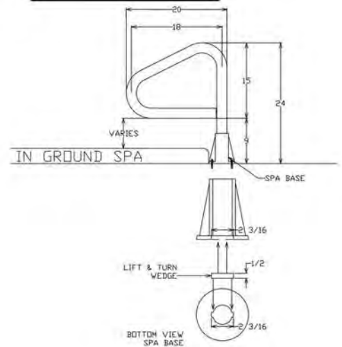
SF-24-LT SPA RAILS
