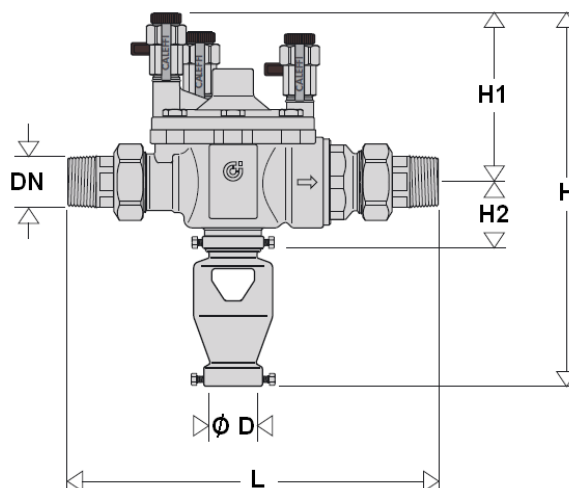
DN 3/4" - 1"
