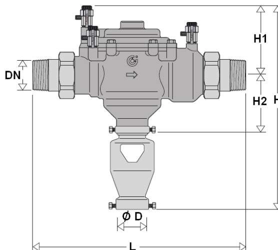
DN 1"1/2 - 2"
