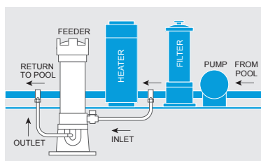
CH200 INSTALLATION OPTIONS
