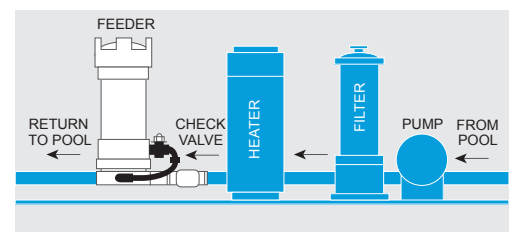
CH100 INSTALLATION
