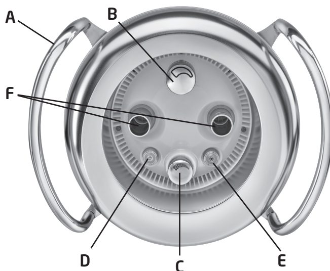
Figure 1 - BaduJet Imperial Deluxe (Front View)
