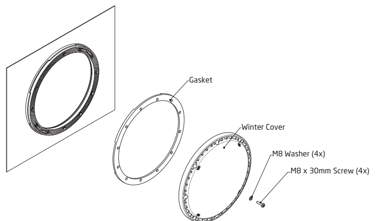
Figure 5 Winter Cover Kit
