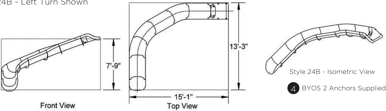
24 LINEAR FEET RIVER RUN Style 24B - Left Turn Shown
