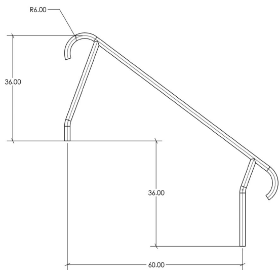
STAIR RAIL (MER-1002)
