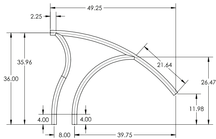
DR-D3D DECK TO DECK RETURN STAIR RAIL
