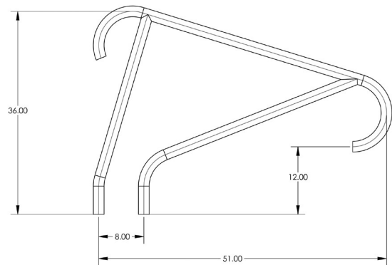
DECK-MOUNTED STAIR RAIL (MER-1004)
