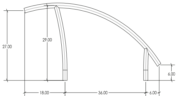
DECK-MOUNTED HANDRAIL (ART-1005)
