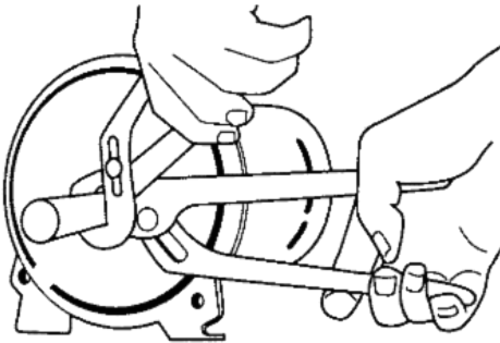
Figure 17: Remove Venturi
