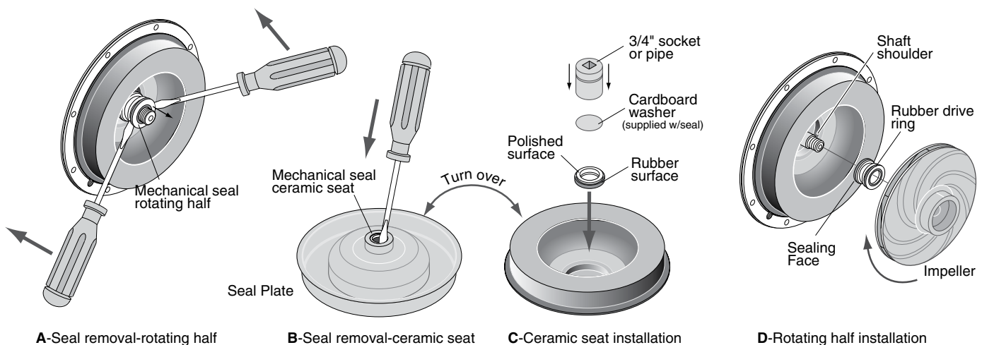
Figure 7: Seal replacement
