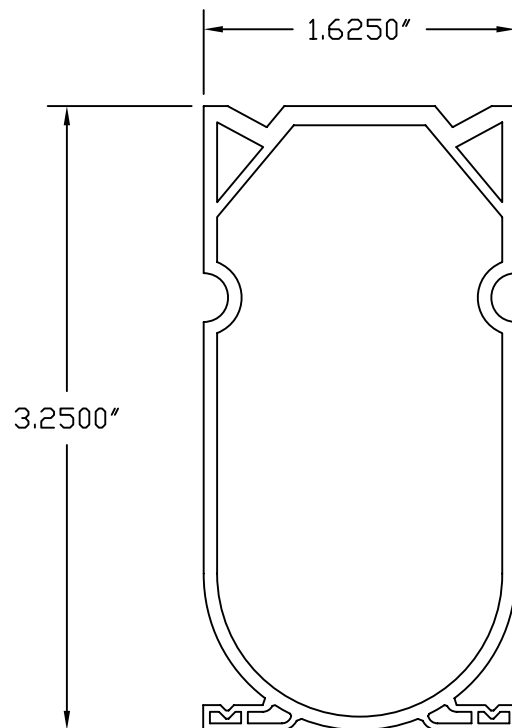
CHANNEL DRAIN
