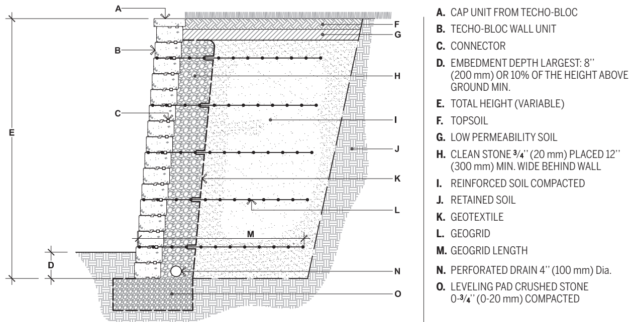
WALL INSTALLATION - GEOGRID REINFORCED WALL Typical cross section
