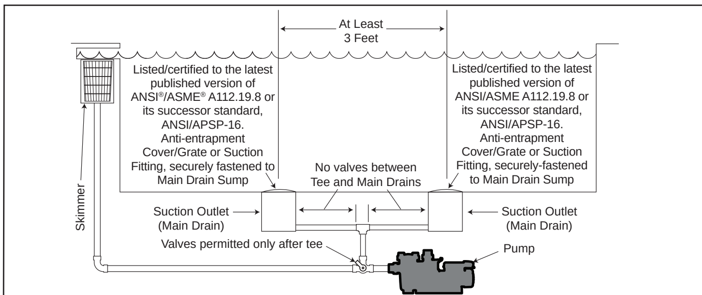
Figure 1. Number of Suction Outlets Per Pump
