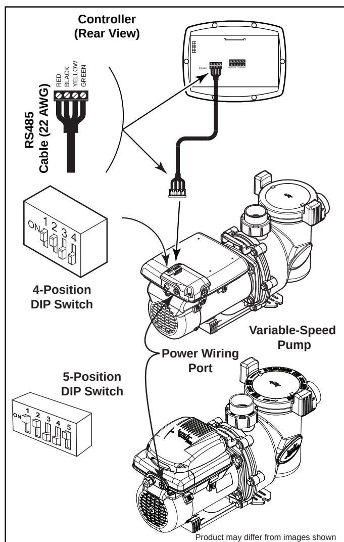
Figure 9. Wiring Variable-Speed Controller (JEP-R)
