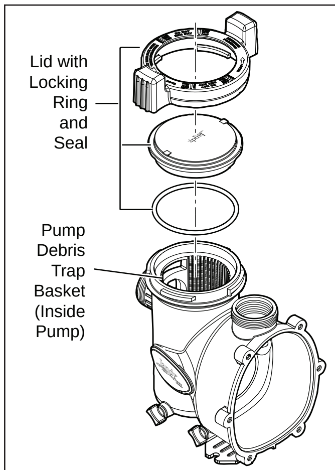
Figure 14. Exploded View of Pump
