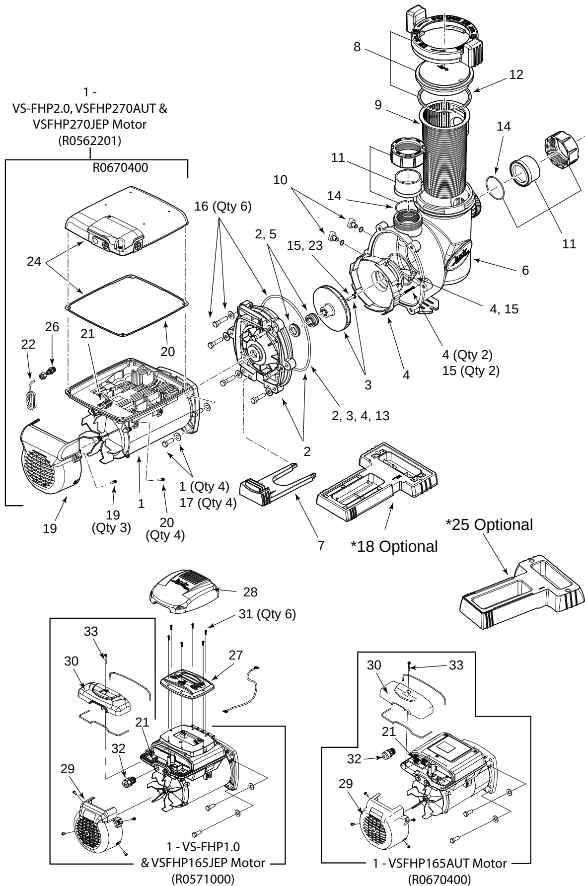
Figure 15. VS FloPro Series Pumps Exploded View
