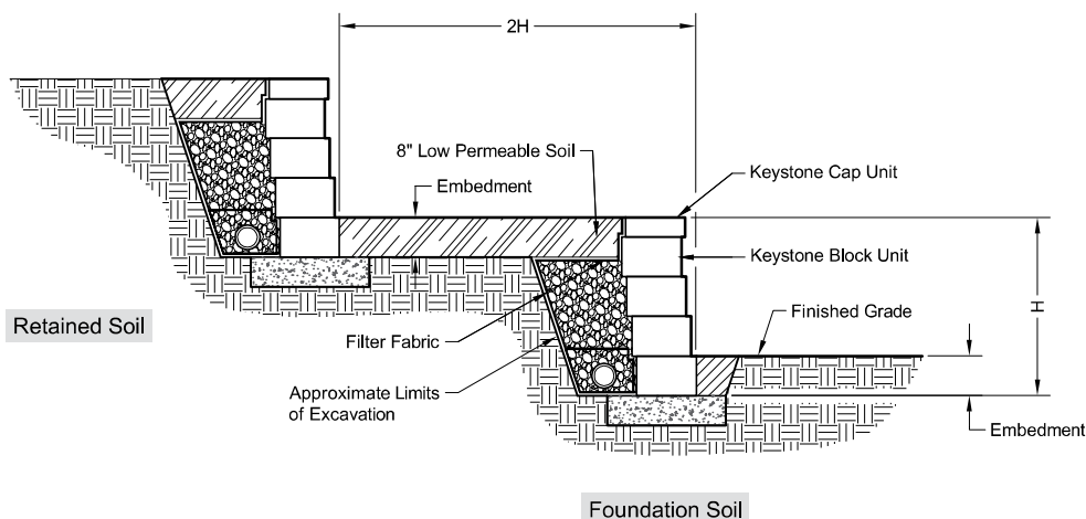
E:11 - INDEPENDENT TIERED GRAVITY WALL
