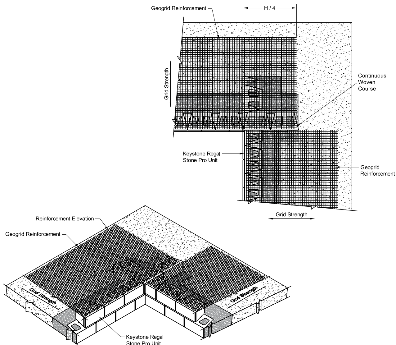
C:10 - TYPICAL ALTERNATING GEOGRID INSTALLATION FOR INSIDE CORNERS (ELEVATION)
