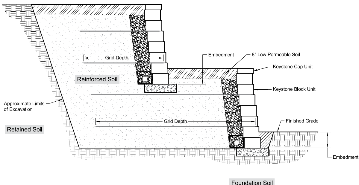
E:12 - TIERED REINFORCED WALL
