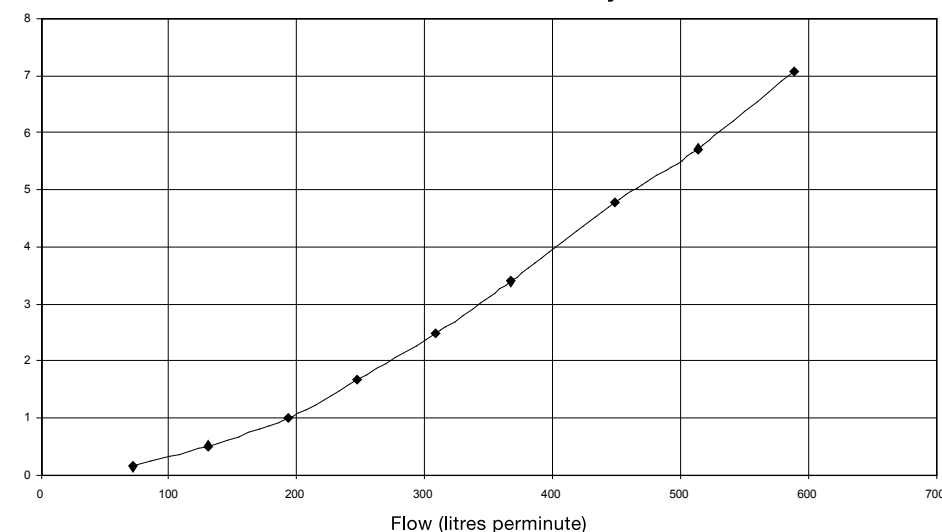
Head Loss Curves on MultiCyclone
