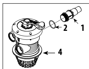
DETAIL 4
