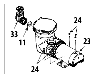
DETAIL 4a
