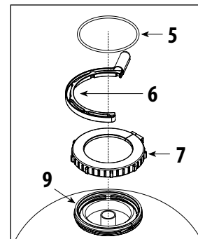
DETAIL 2
