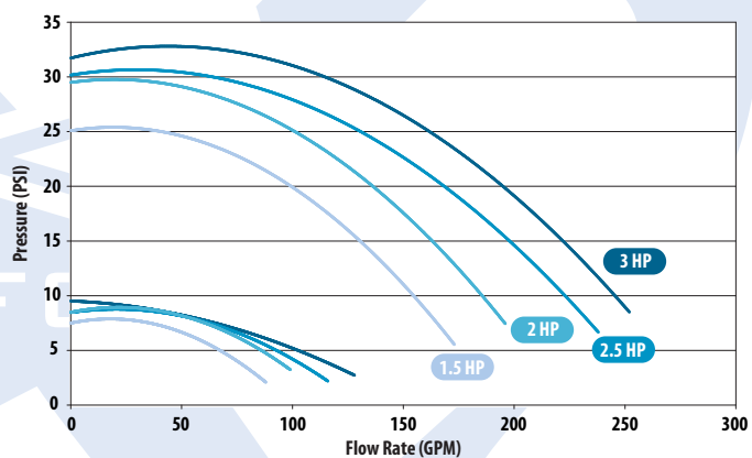
EX2 Performance Chart
